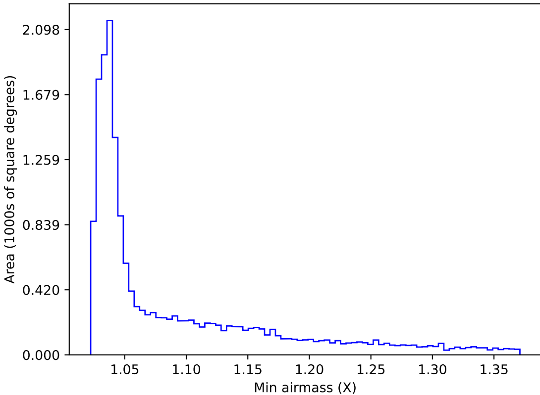
noroll_mjdp180_v3.4_10yrs WFD g band: Min airmass
