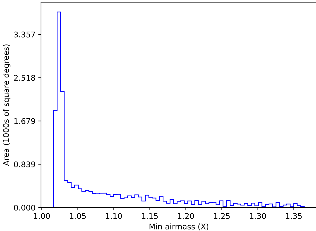
noroll_mjdp180_v3.4_10yrs WFD all bands: Min airmass
