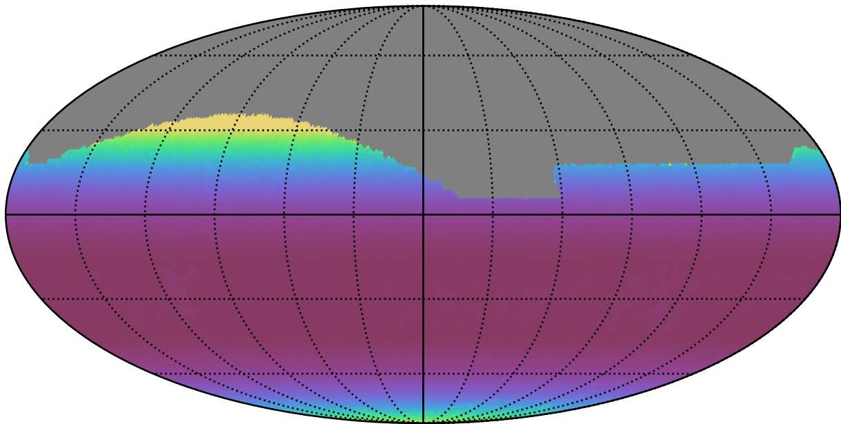
noroll_mjdp180_v3.4_10yrs All sky z band: Min airmass
