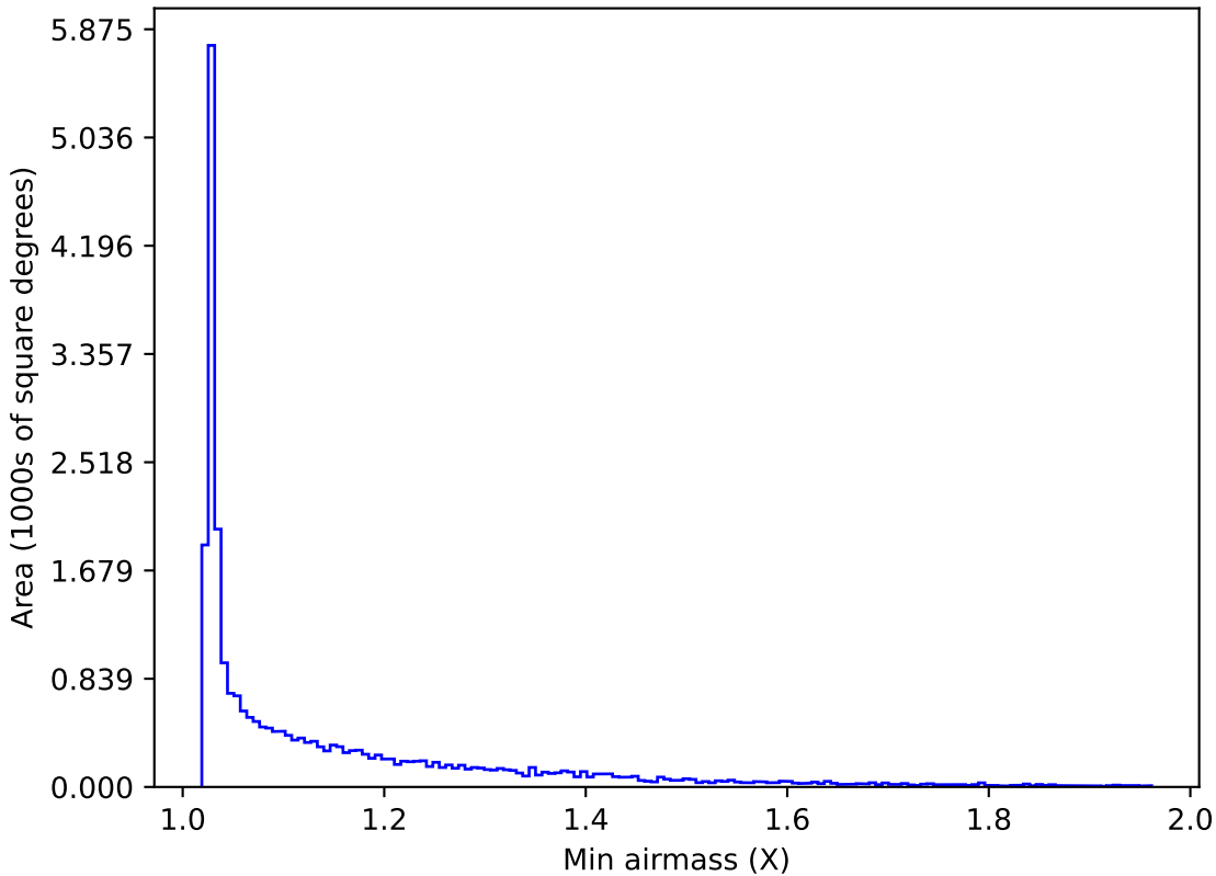
noroll_mjdp180_v3.4_10yrs All sky z band: Min airmass
