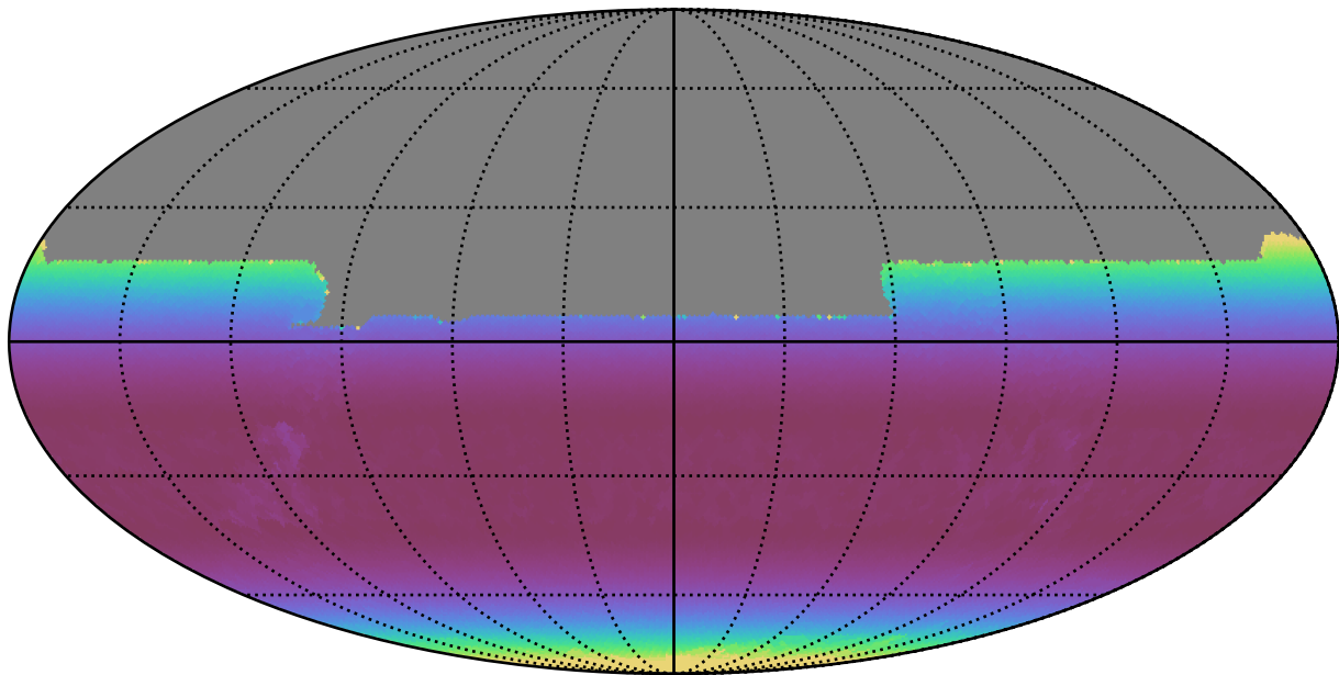
noroll_mjdp180_v3.4_10yrs All sky y band: Min airmass
