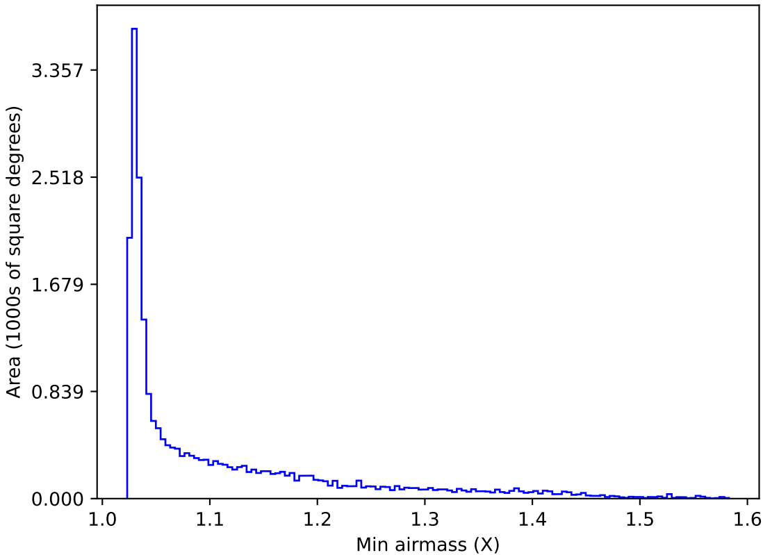
noroll_mjdp180_v3.4_10yrs All sky y band: Min airmass
