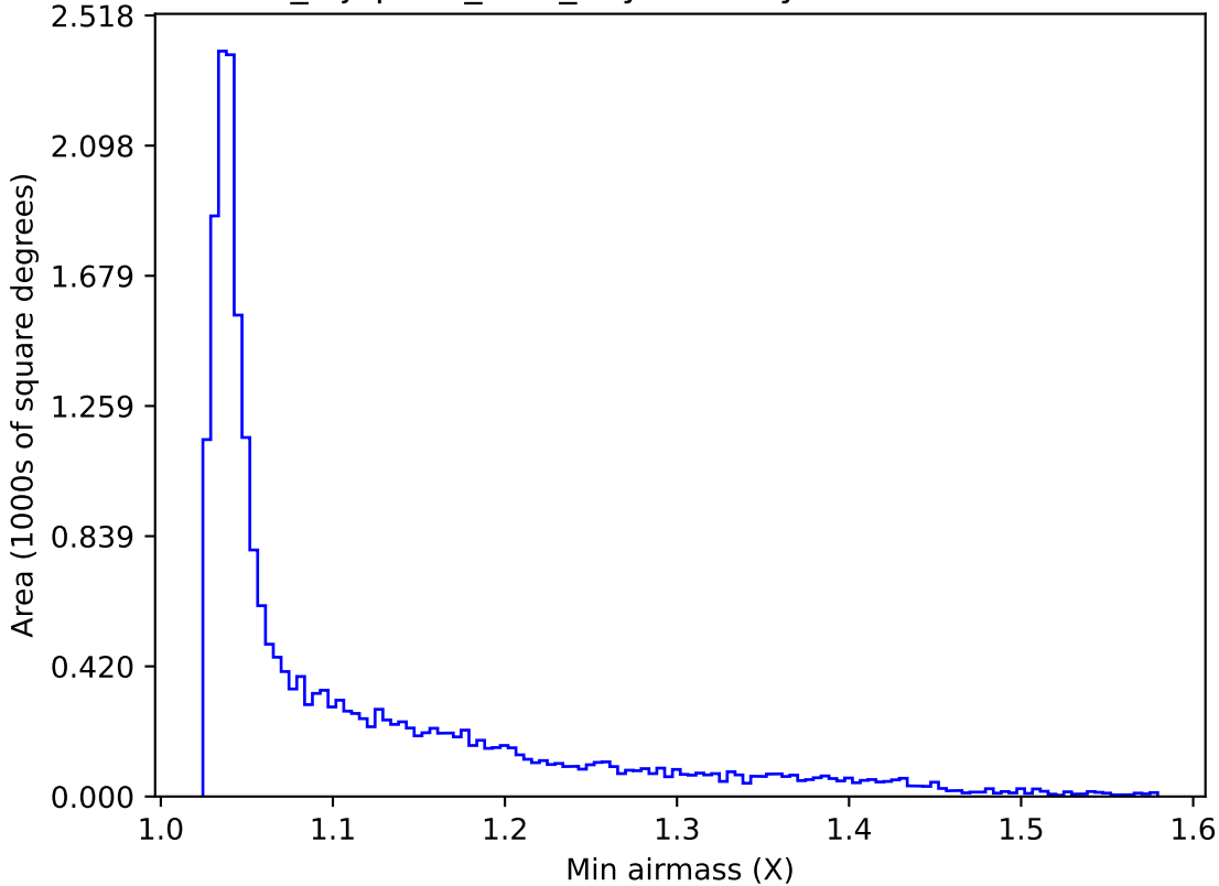
noroll_mjdp180_v3.4_10yrs All sky u band: Min airmass
