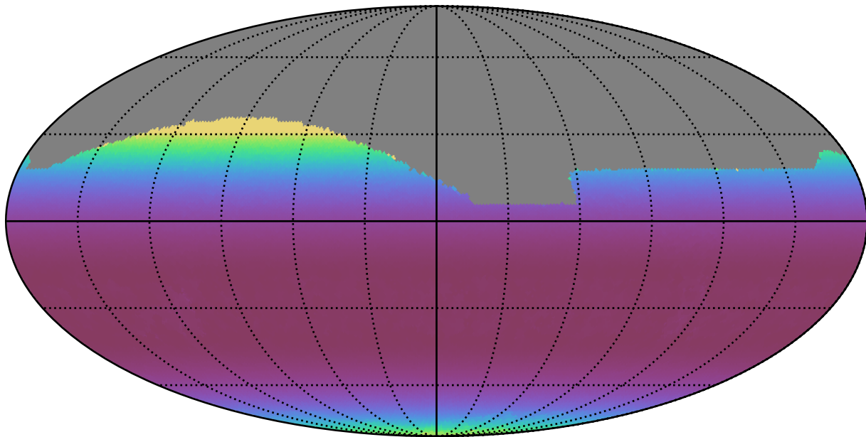
noroll_mjdp180_v3.4_10yrs All sky r band: Min airmass
