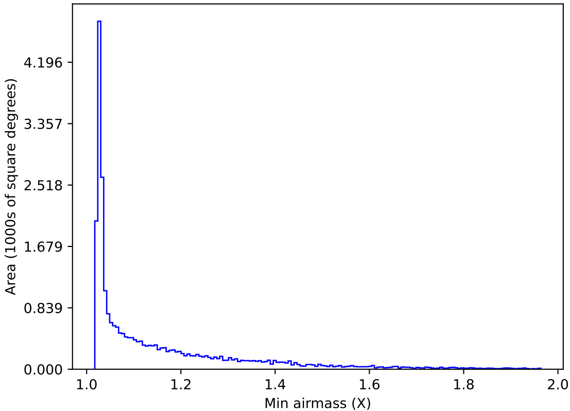
noroll_mjdp180_v3.4_10yrs All sky r band: Min airmass
