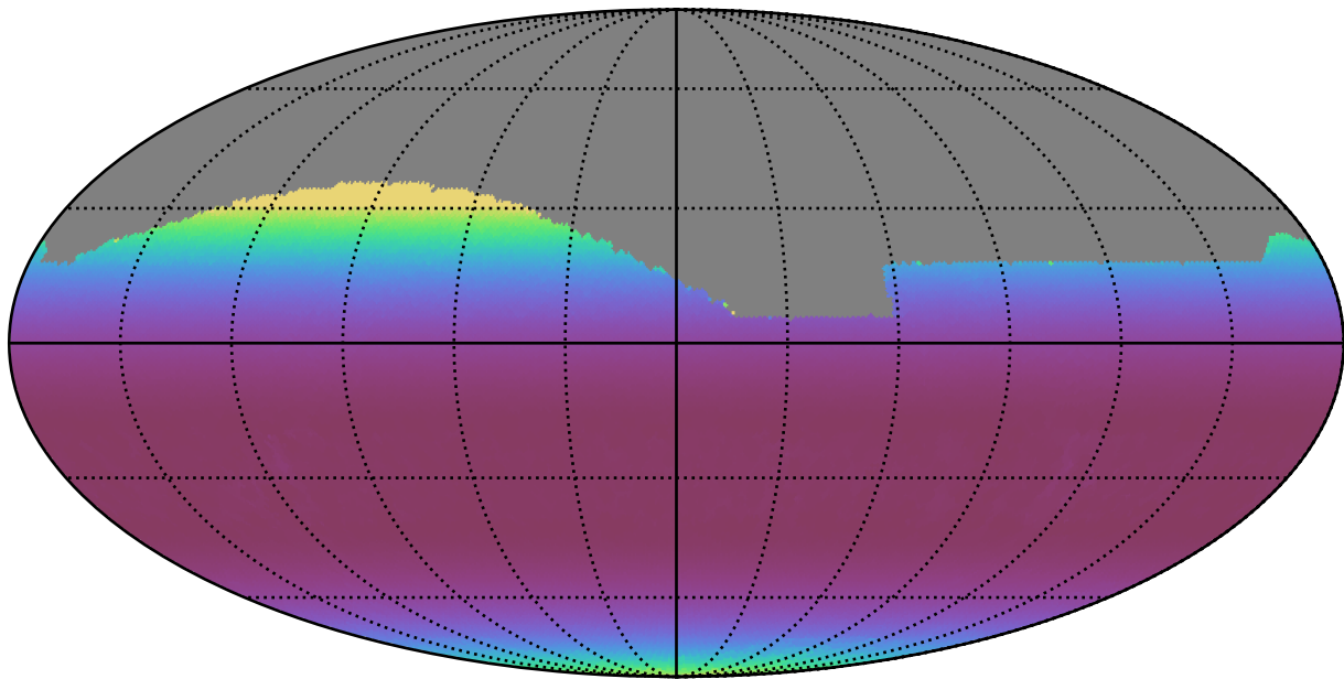
noroll_mjdp180_v3.4_10yrs All sky i band: Min airmass
