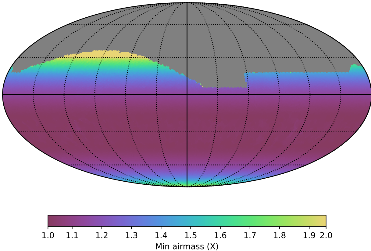
noroll_mjdp180_v3.4_10yrs All sky i band: Min airmass
