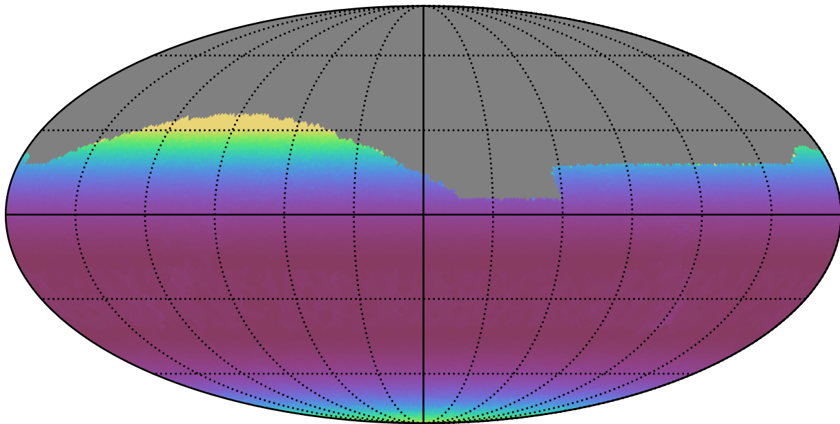
noroll_mjdp180_v3.4_10yrs All sky g band: Min airmass
