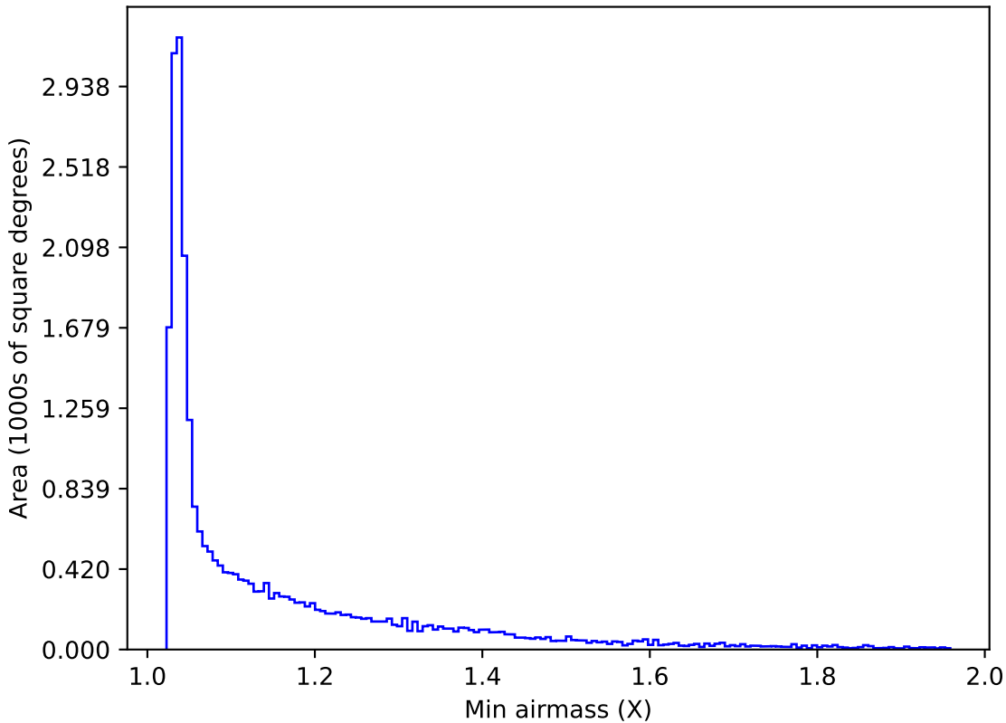
noroll_mjdp180_v3.4_10yrs All sky g band: Min airmass
