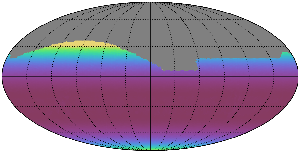
noroll_mjdp180_v3.4_10yrs All sky all bands: Min airmass
