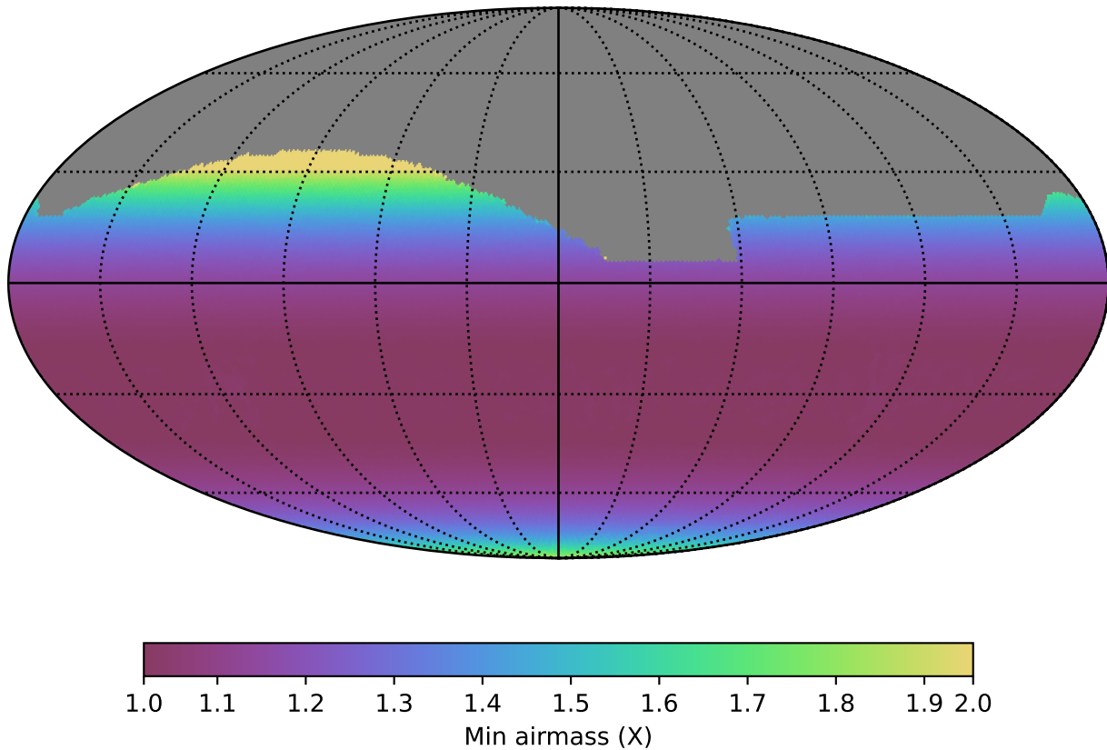
noroll_mjdp180_v3.4_10yrs All sky all bands: Min airmass
