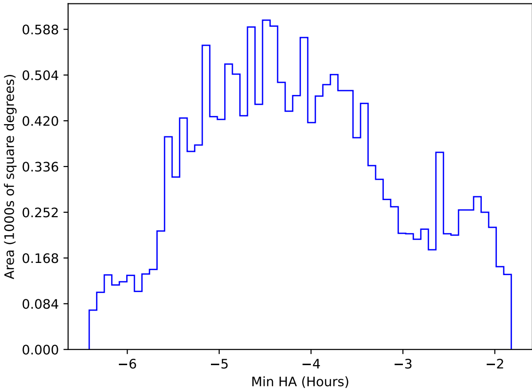
noroll_mjdp180_v3.4_10yrs WFD z band: Min HA
