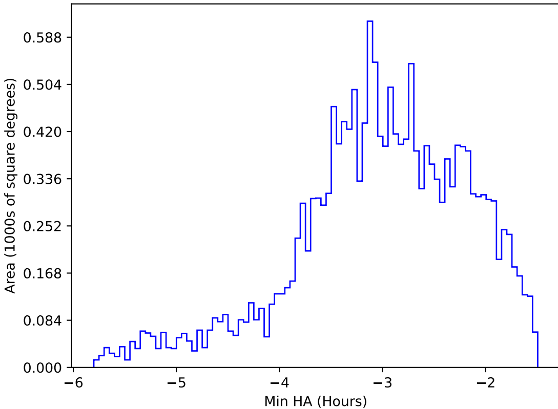
noroll_mjdp180_v3.4_10yrs WFD u band: Min HA
