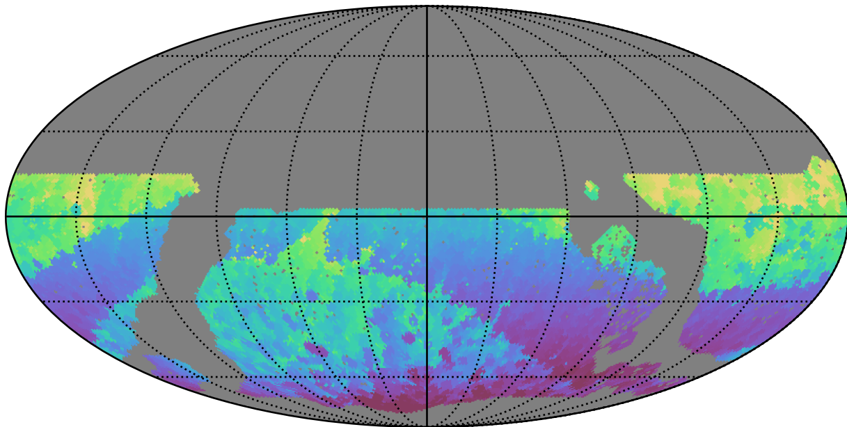
noroll_mjdp180_v3.4_10yrs WFD r band: Min HA
