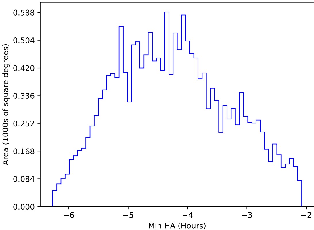
noroll_mjdp180_v3.4_10yrs WFD r band: Min HA
