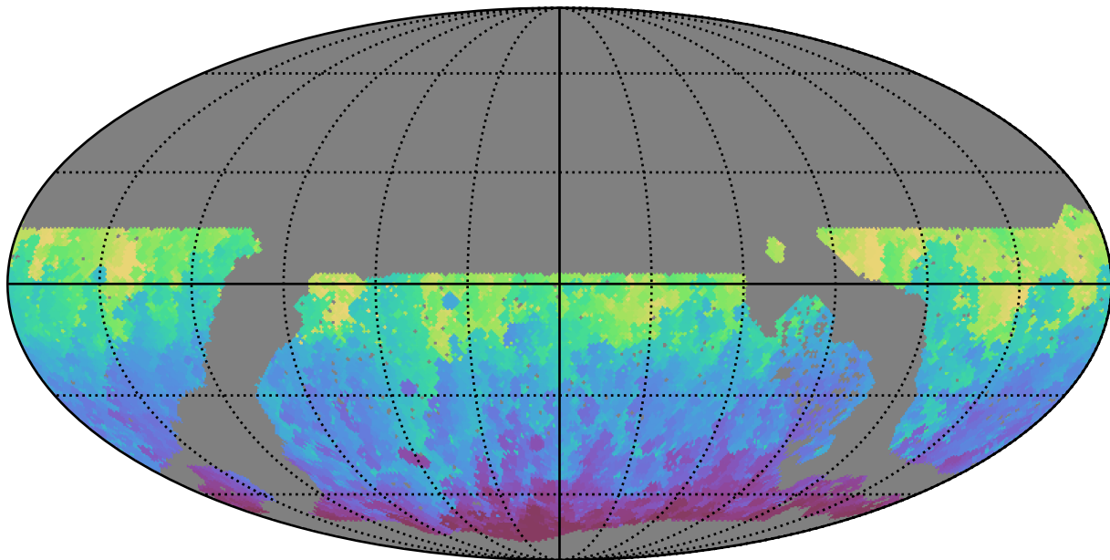
noroll_mjdp180_v3.4_10yrs WFD g band: Min HA
