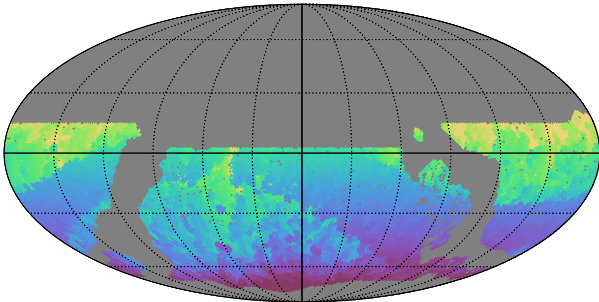
noroll_mjdp180_v3.4_10yrs WFD all bands: Min HA
