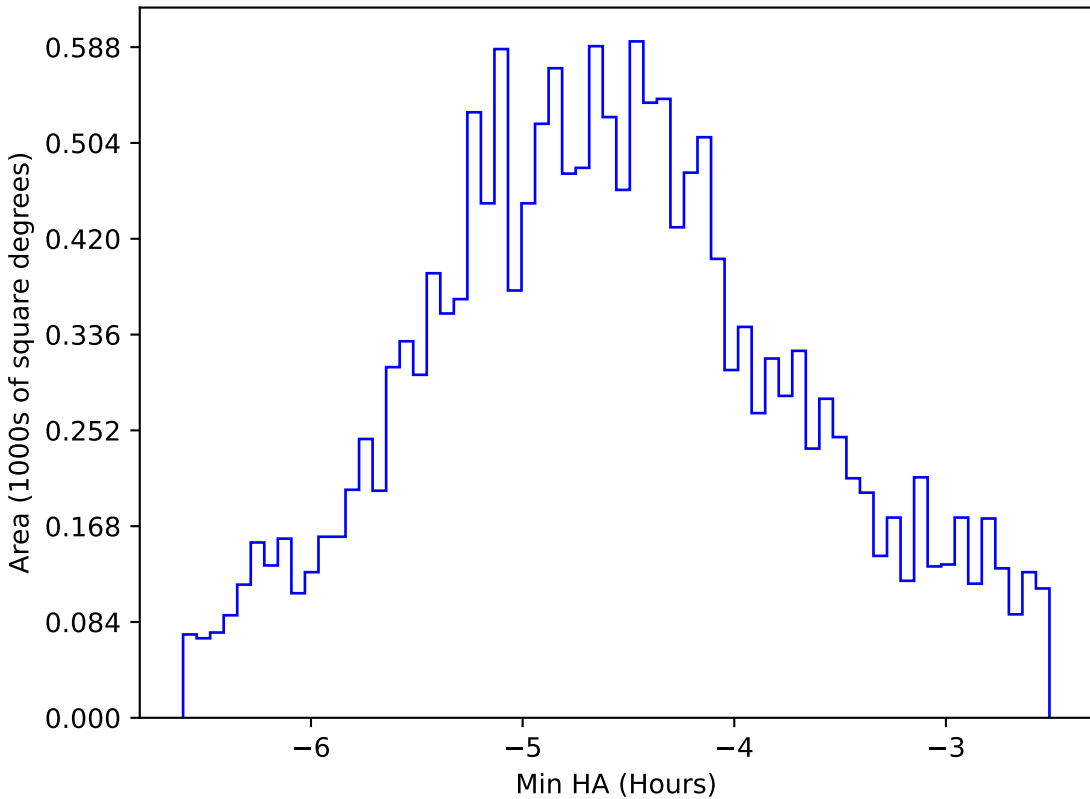
noroll_mjdp180_v3.4_10yrs WFD all bands: Min HA
