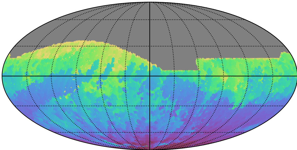
noroll_mjdp180_v3.4_10yrs All sky z band: Min HA
