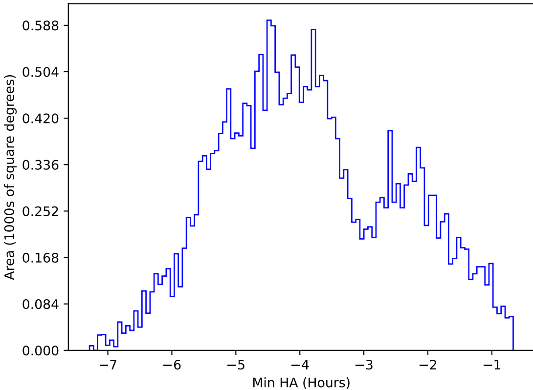
noroll_mjdp180_v3.4_10yrs All sky z band: Min HA
