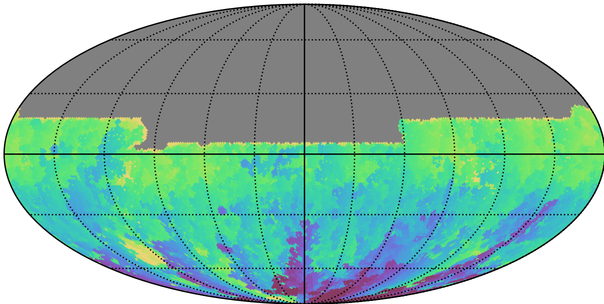
noroll_mjdp180_v3.4_10yrs All sky u band: Min HA
