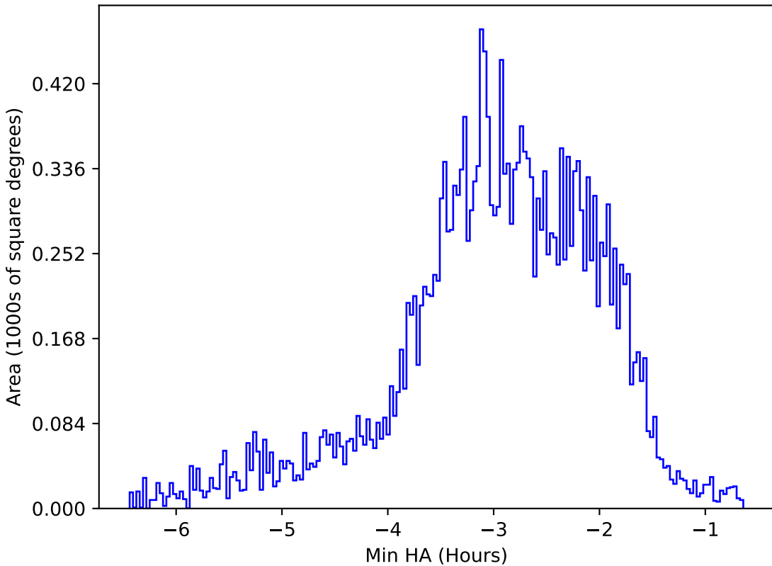
noroll_mjdp180_v3.4_10yrs All sky u band: Min HA
