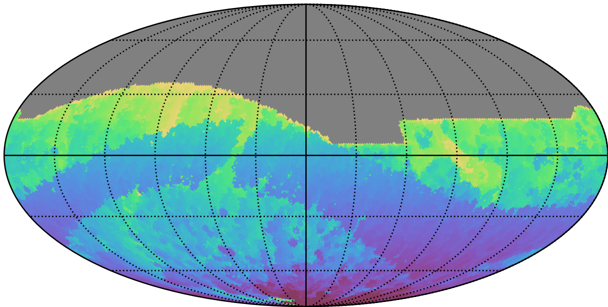
noroll_mjdp180_v3.4_10yrs All sky r band: Min HA
