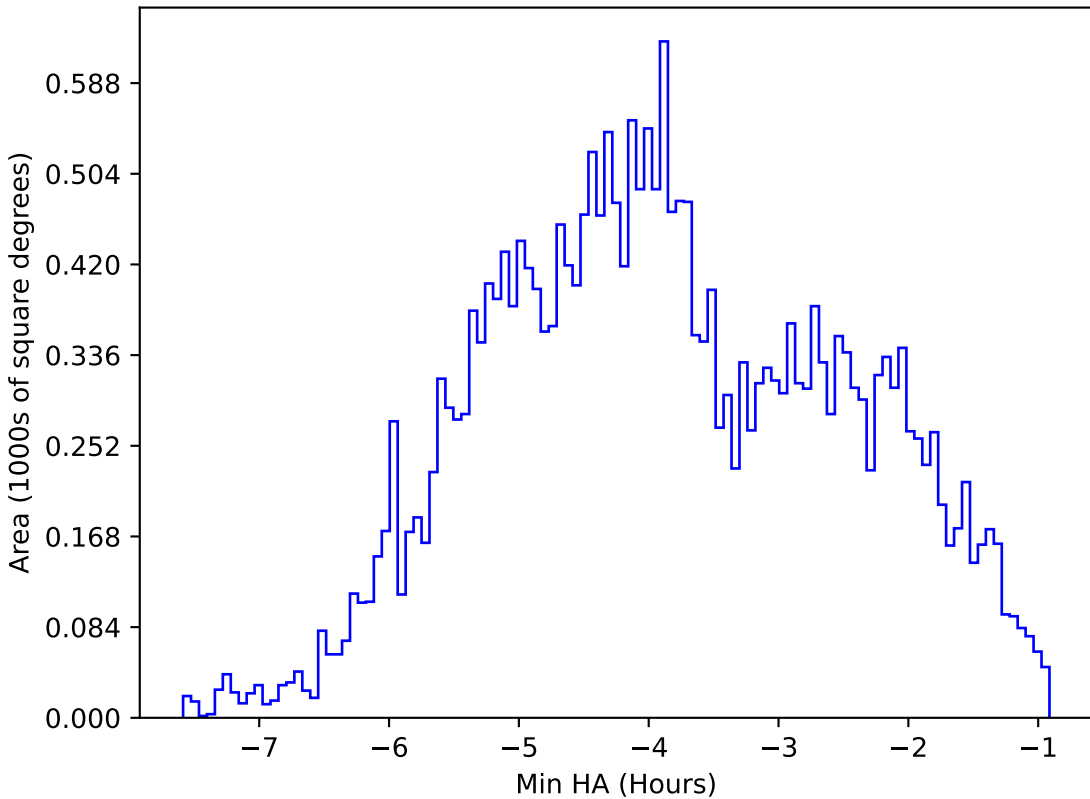
noroll_mjdp180_v3.4_10yrs All sky i band: Min HA
