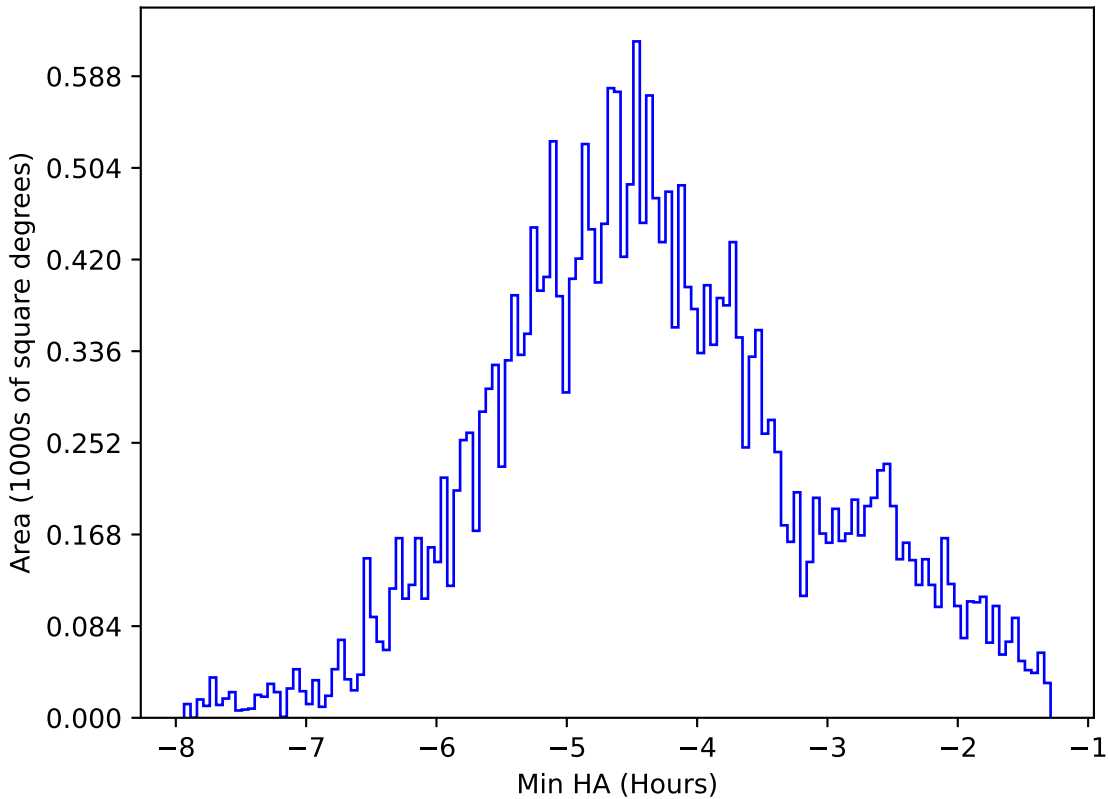
noroll_mjdp180_v3.4_10yrs All sky all bands: Min HA
