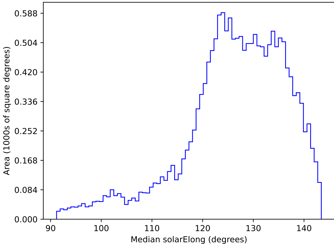
noroll_mjdp180_v3.4_10yrs WFD z band: Median solarElong
