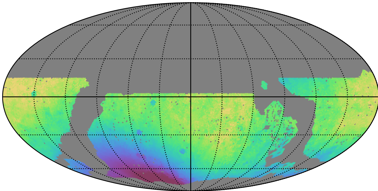
noroll_mjdp180_v3.4_10yrs WFD r band: Median solarElong
