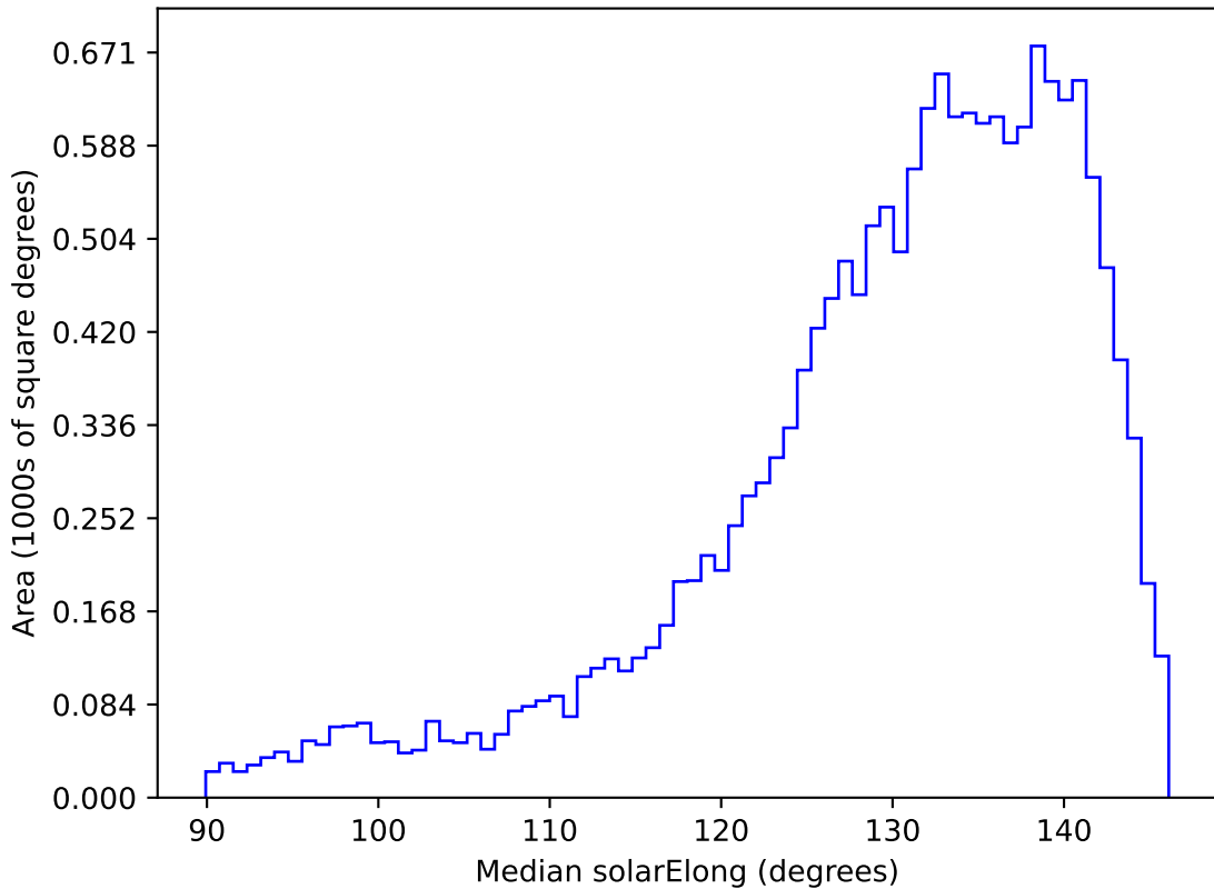
noroll_mjdp180_v3.4_10yrs WFD r band: Median solarElong
