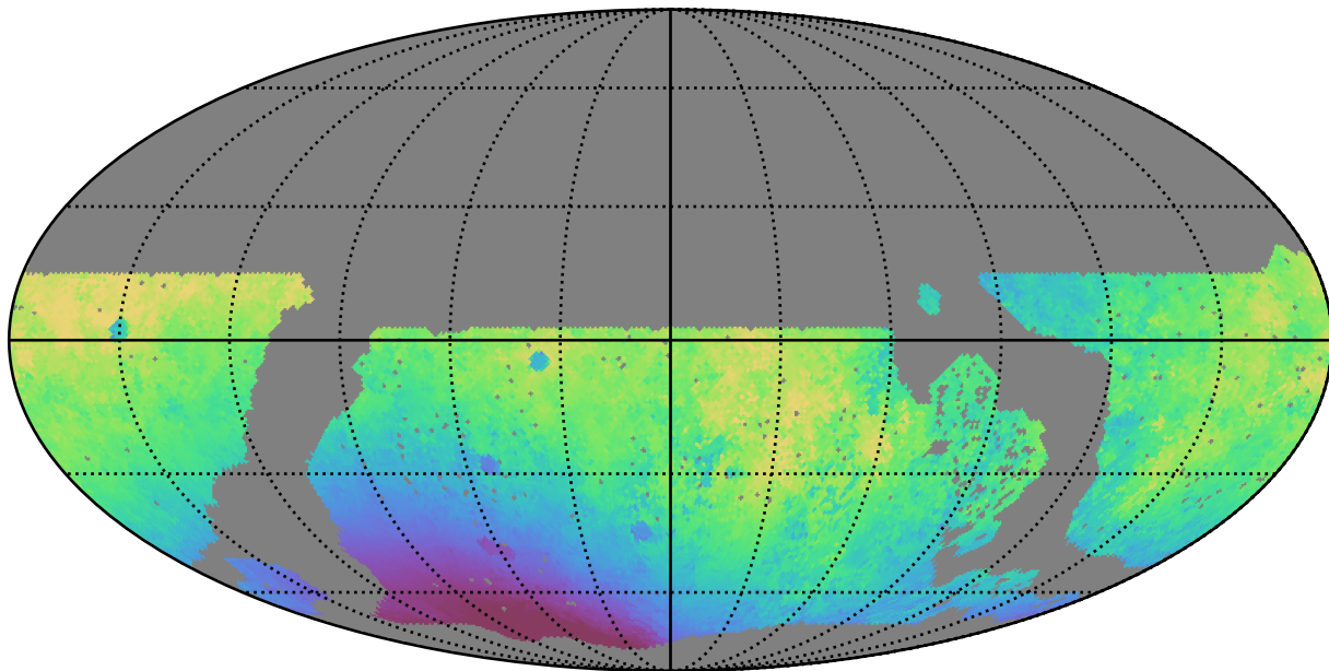
noroll_mjdp180_v3.4_10yrs WFD g band: Median solarElong
