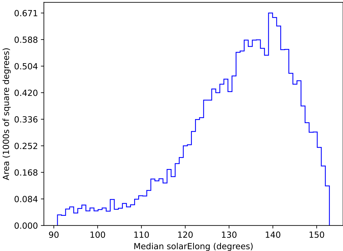
noroll_mjdp180_v3.4_10yrs WFD g band: Median solarElong
