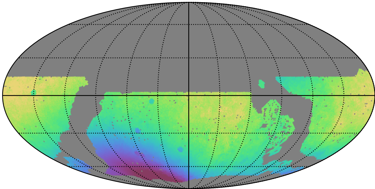
noroll_mjdp180_v3.4_10yrs WFD all bands: Median solarElong
