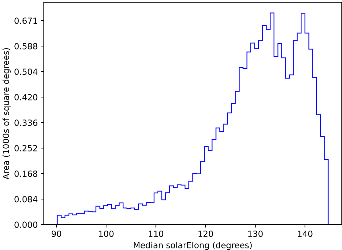
noroll_mjdp180_v3.4_10yrs WFD all bands: Median solarElong
