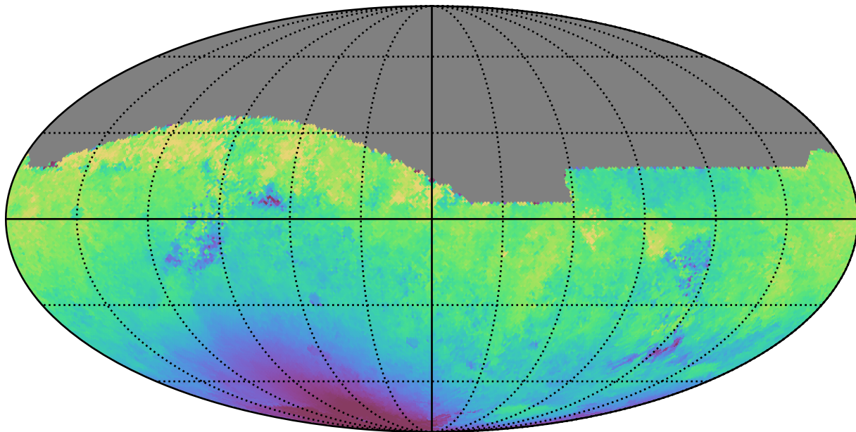
noroll_mjdp180_v3.4_10yrs All sky z band: Median solarElong
