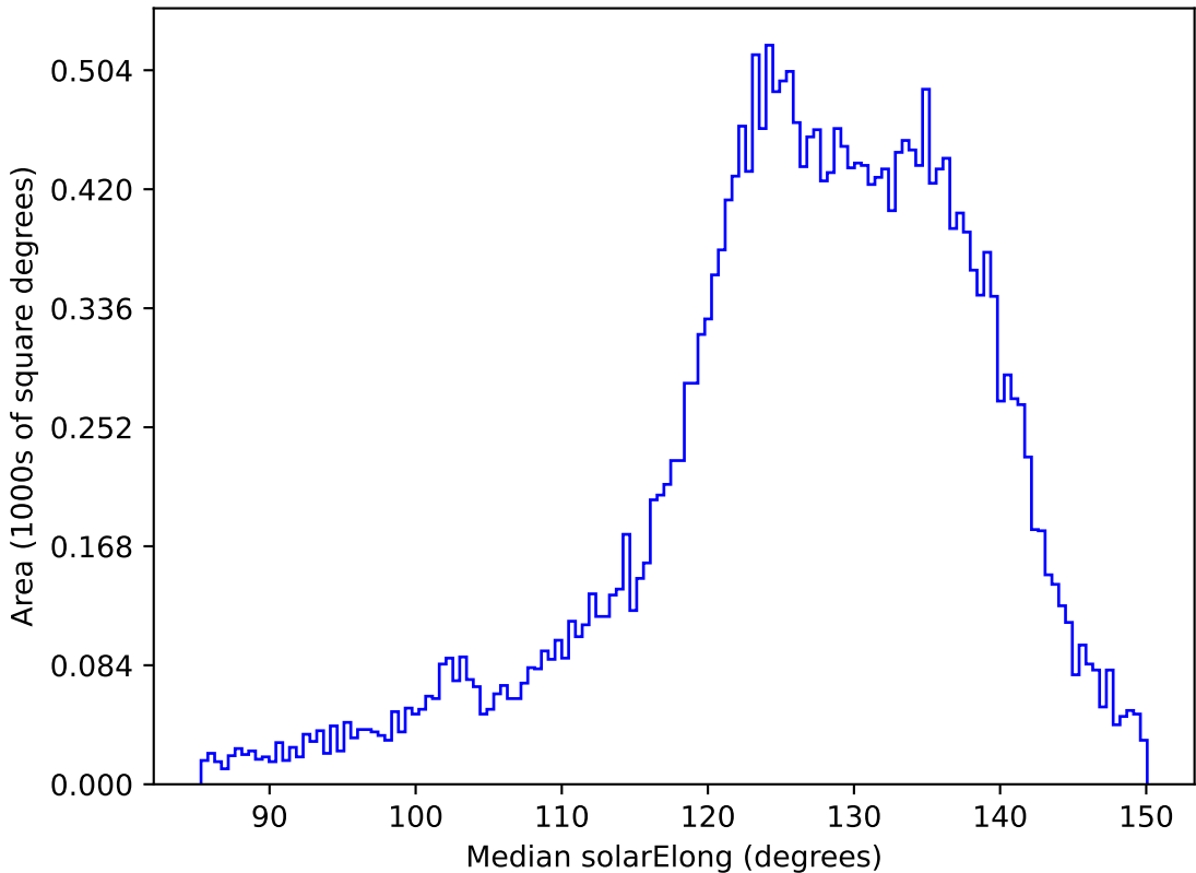
noroll_mjdp180_v3.4_10yrs All sky z band: Median solarElong
