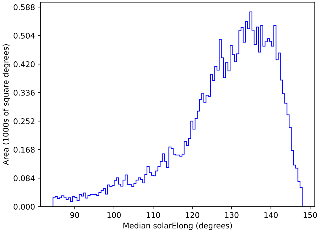
noroll_mjdp180_v3.4_10yrs All sky y band: Median solarElong
