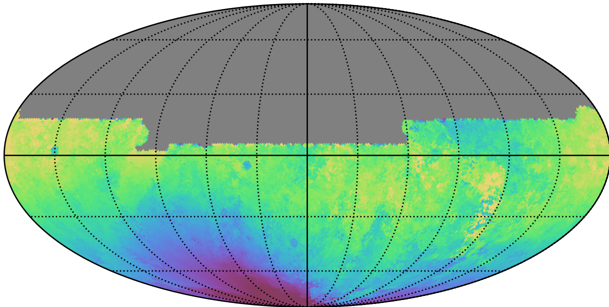
noroll_mjdp180_v3.4_10yrs All sky u band: Median solarElong
