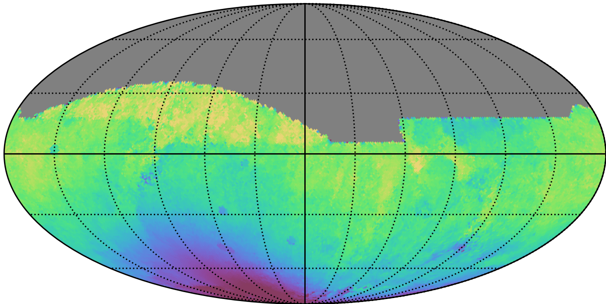
noroll_mjdp180_v3.4_10yrs All sky i band: Median solarElong
