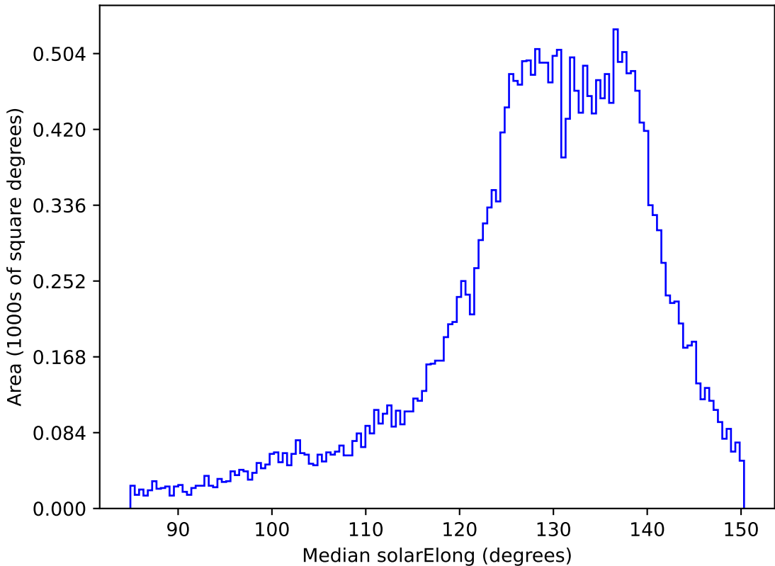
noroll_mjdp180_v3.4_10yrs All sky i band: Median solarElong
