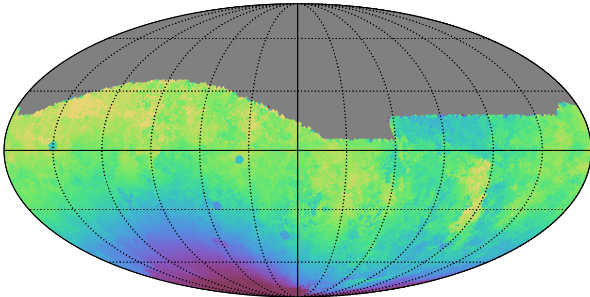
noroll_mjdp180_v3.4_10yrs All sky g band: Median solarElong
