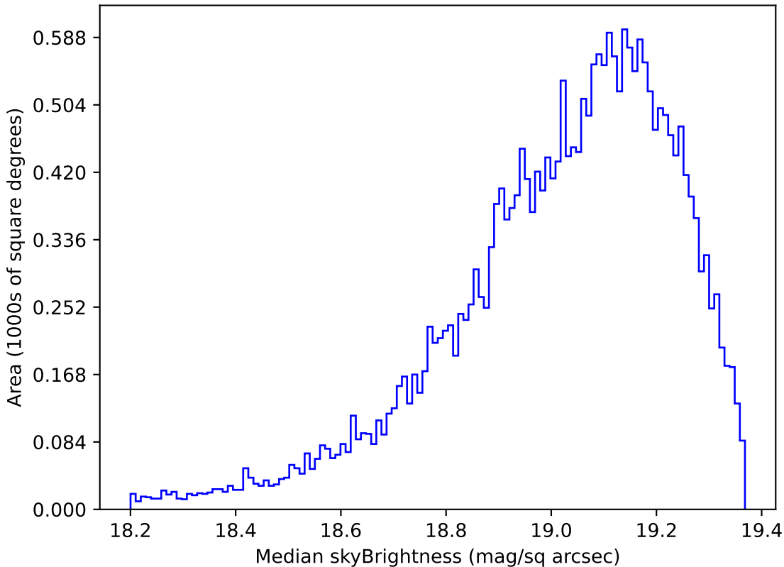
noroll_mjdp180_v3.4_10yrs Yr 1 z band: Median skyBrightness
