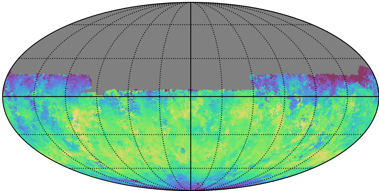
noroll_mjdp180_v3.4_10yrs Yr 1 y band: Median skyBrightness
