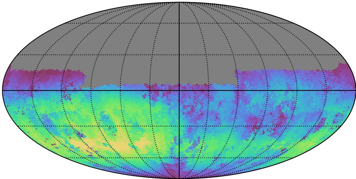
noroll_mjdp180_v3.4_10yrs Yr 1 u band: Median skyBrightness
