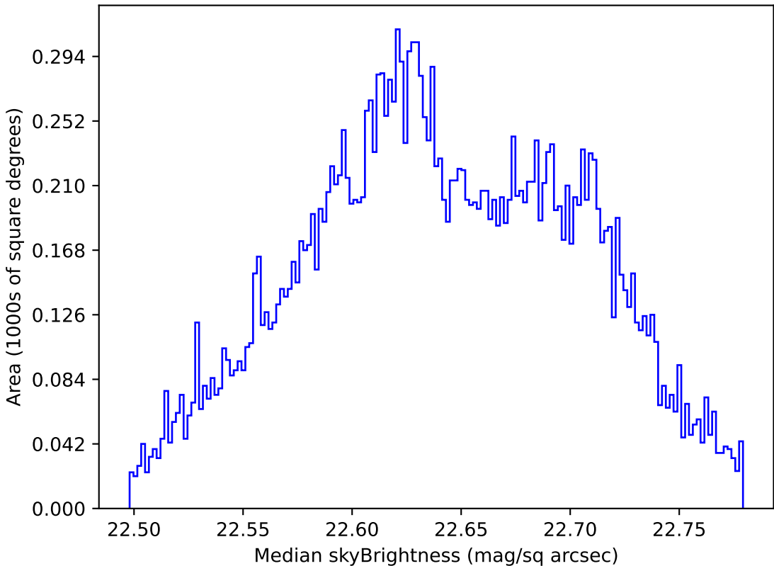
noroll_mjdp180_v3.4_10yrs Yr 1 u band: Median skyBrightness
