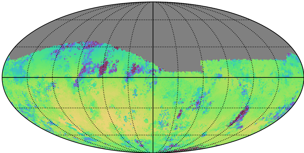
noroll_mjdp180_v3.4_10yrs Yr 1 r band: Median skyBrightness
