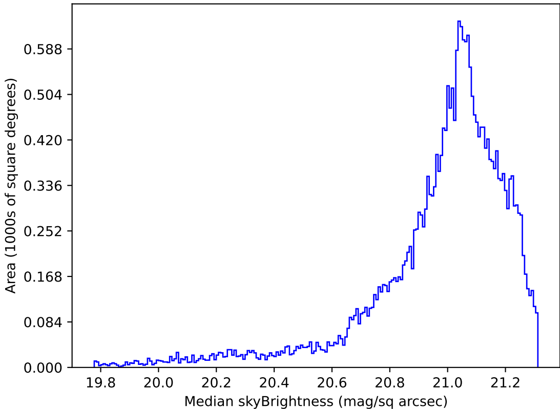
noroll_mjdp180_v3.4_10yrs Yr 1 r band: Median skyBrightness
