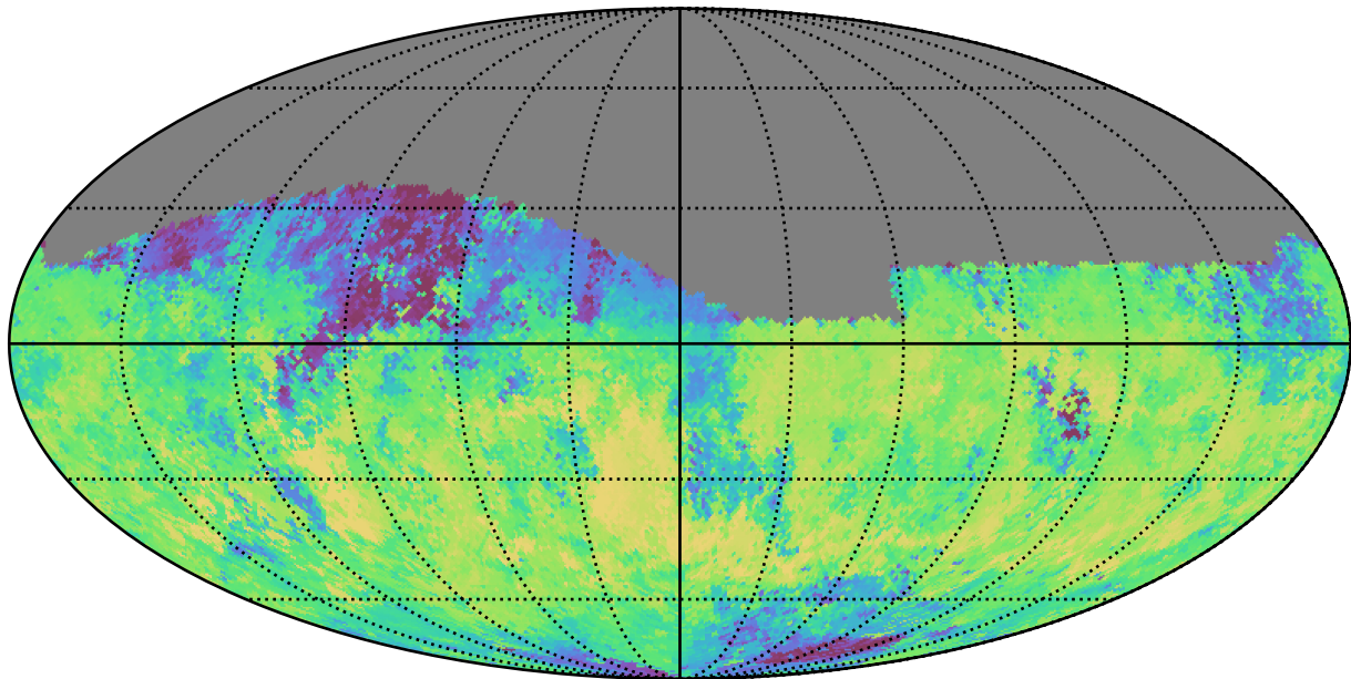
noroll_mjdp180_v3.4_10yrs Yr 1 i band: Median skyBrightness
