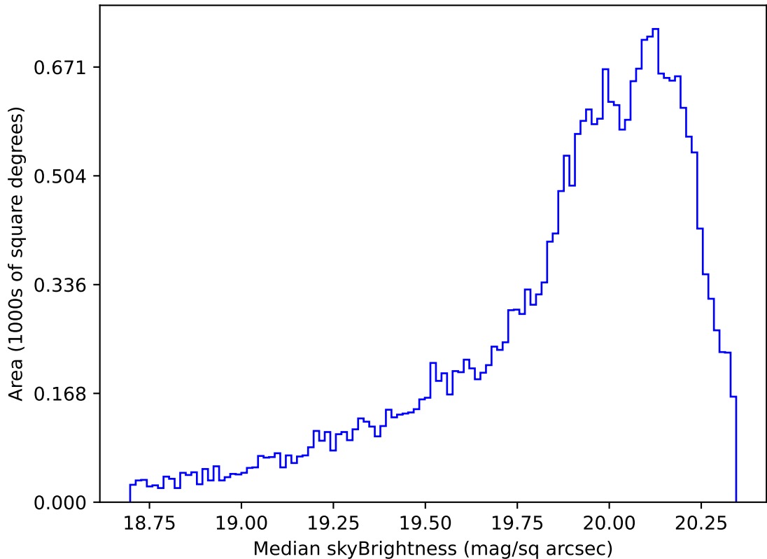
noroll_mjdp180_v3.4_10yrs Yr 1 i band: Median skyBrightness
