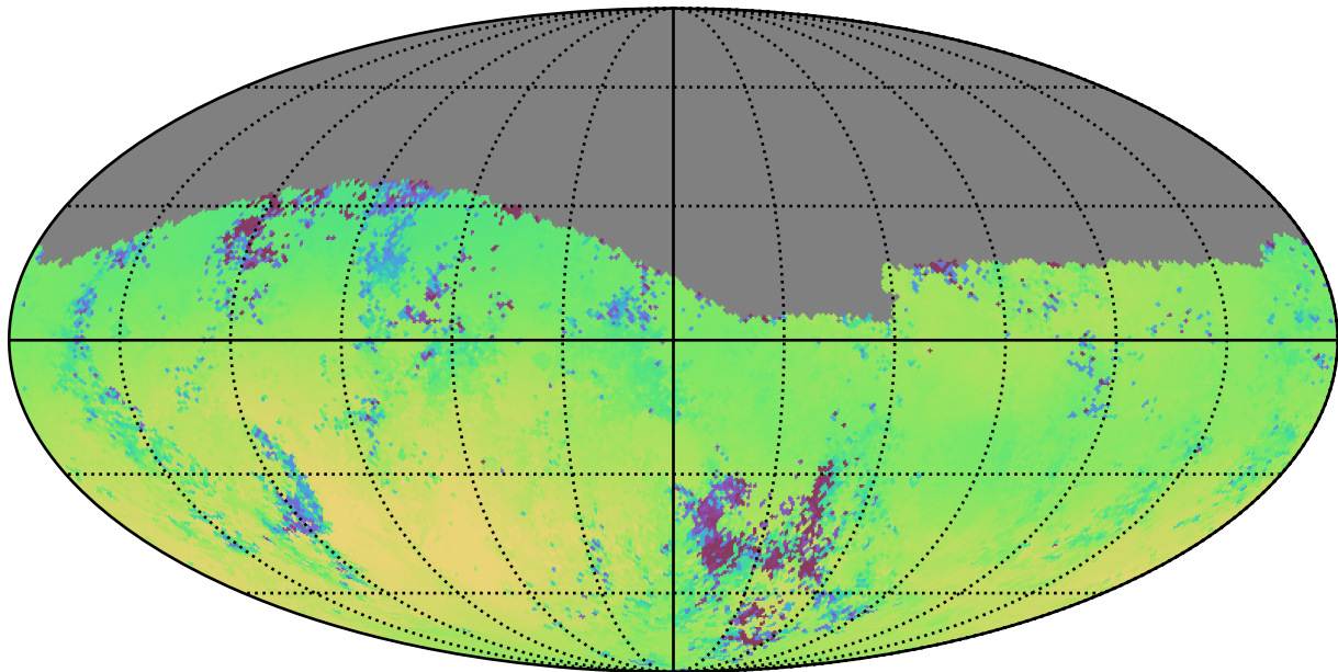
noroll_mjdp180_v3.4_10yrs Yr 1 g band: Median skyBrightness
